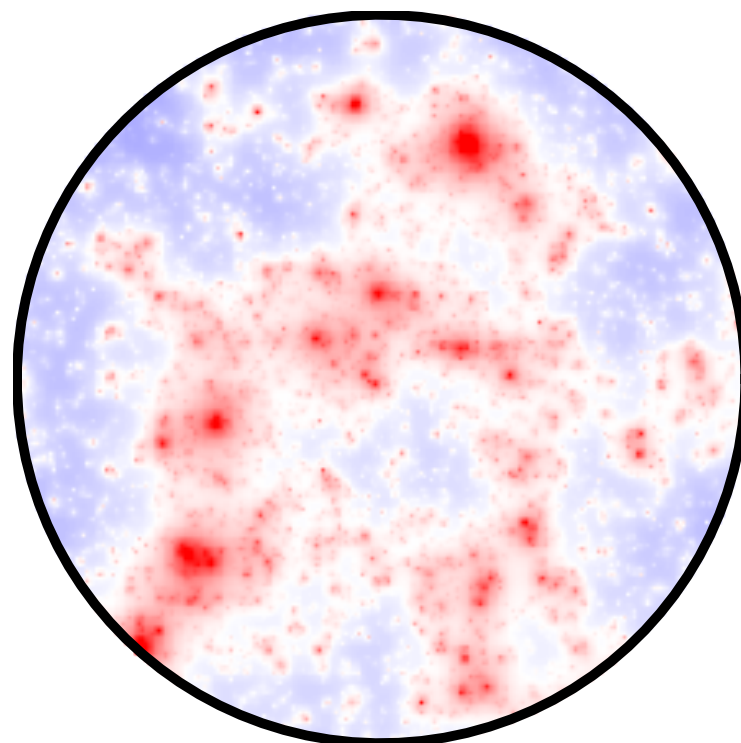
K_{\text{sub}} (multi – plane Born)
