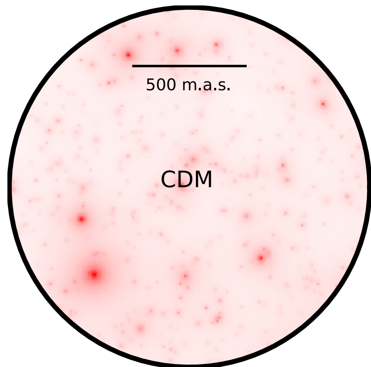
K_{\text{sub}} (single plane)
