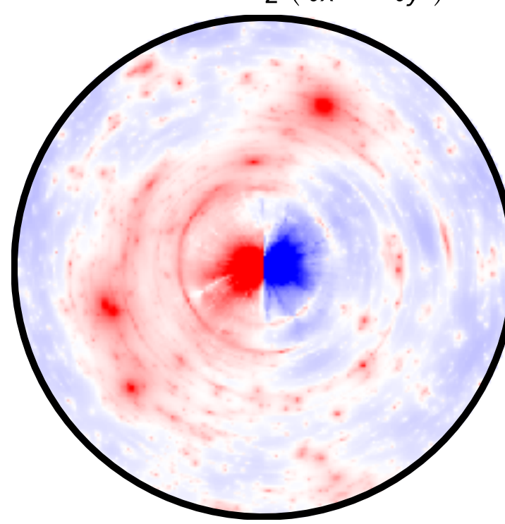
K_{\text{sub}}(\text{effective}) \equiv \frac{1}{2} \left( \frac{\partial \alpha_x}{\partial x} + \frac{\partial \alpha_y}{\partial y} \right) - K_{\text{macro}}
