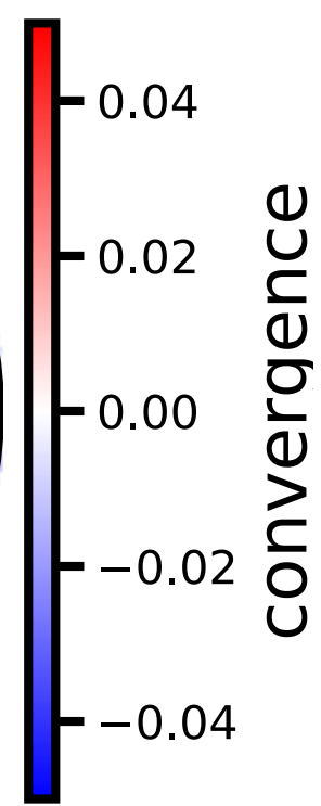
K_{\text{sub}}(\text{effective}) \equiv \frac{1}{2} \left( \frac{\partial \alpha_x}{\partial x} + \frac{\partial \alpha_y}{\partial y} \right) - K_{\text{macro}}
